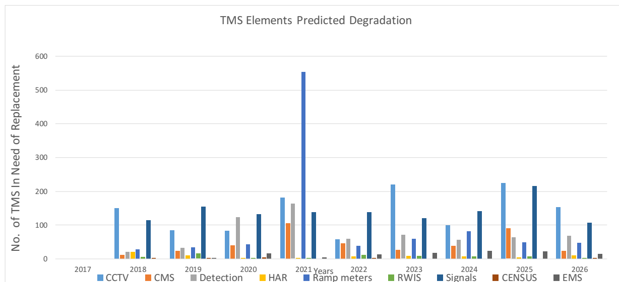
Figure 4-3. Estimate of TMS Elements in Need of Replacement over the next 10 Years
