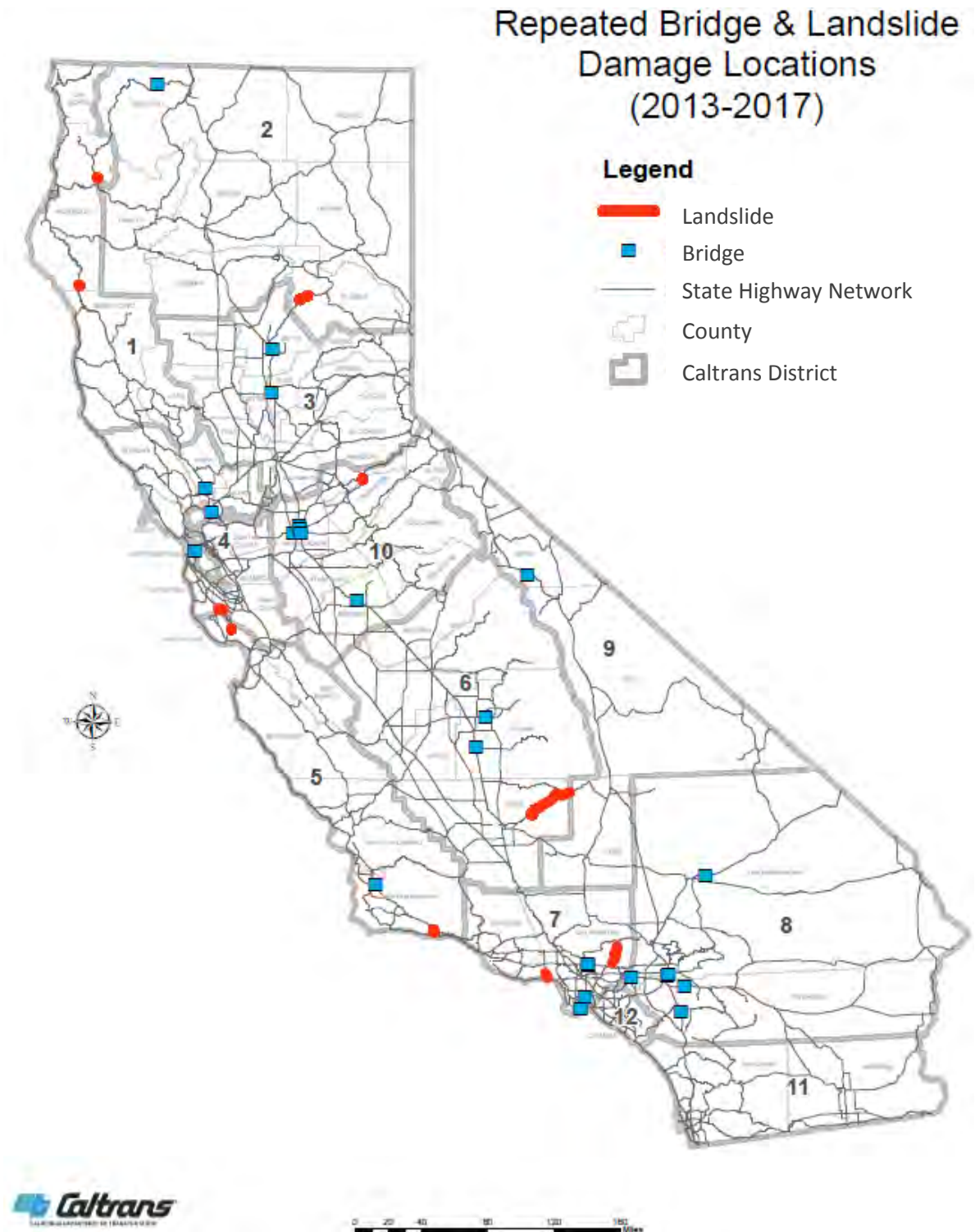
Figure 8-8. Repeated Bridge and Landslide Damage Locations
