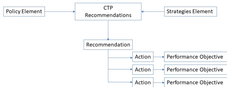
FIGURE 1 RECOMMENDATIONS FRAMEWORK
