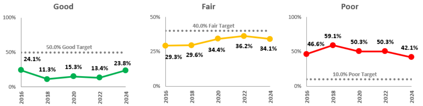
Figure 21 – Condition of Drainage Pump Plants
