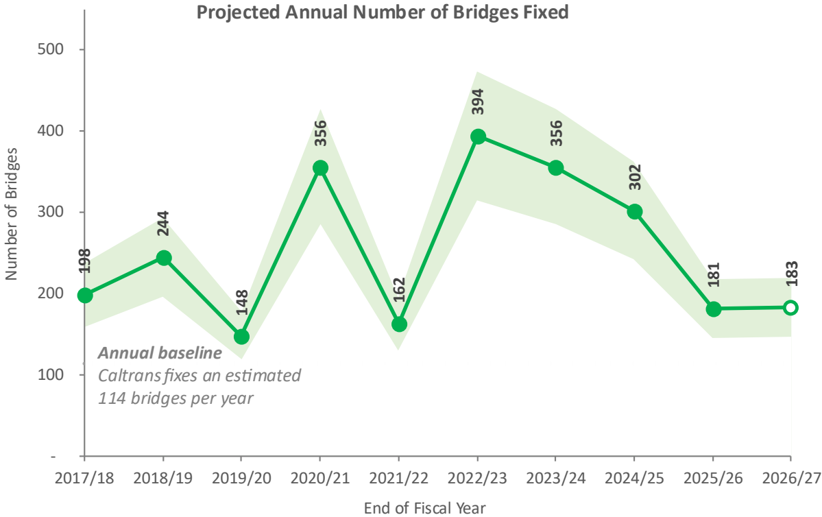
Figure 19 – Projected Number of Bridges Fixed Each Year
