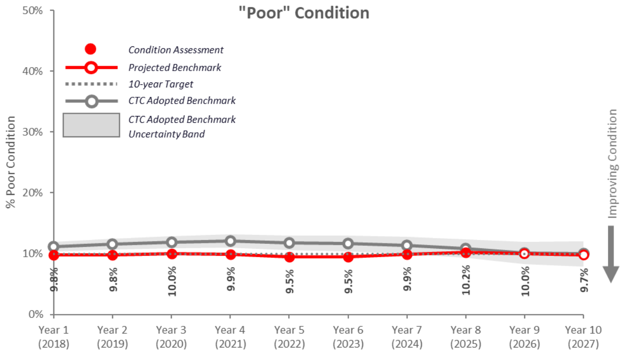
Figure 15 - Drainage, Poor
