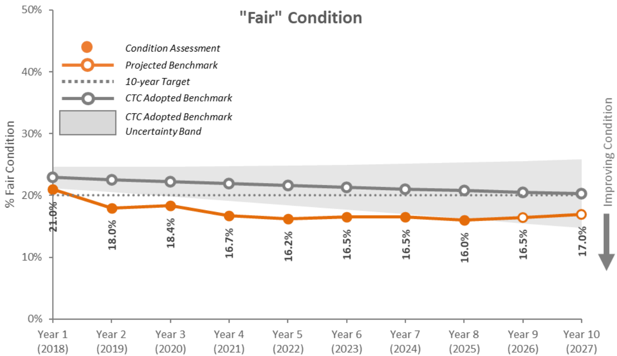
Figure 14 - Drainage, Fair
