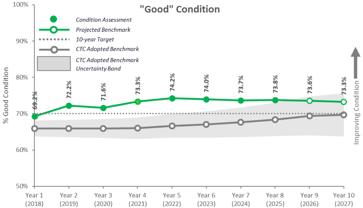
Figure 13 – Drainage, Good
