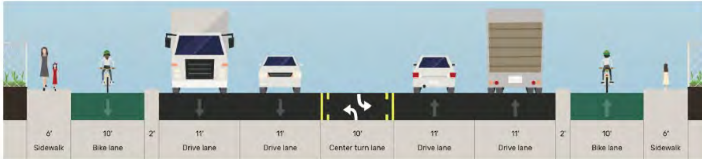
FIGURE 5: ALTERNATIVE 1 CROSS SECTION
